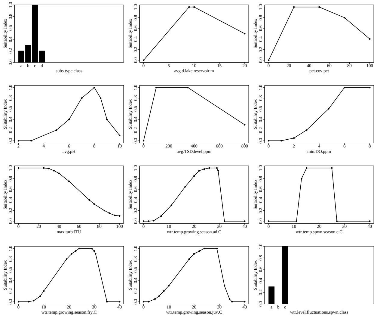
Figure 1. Suitability index graphs for variables included in the smallmouthbassLac model in ecorest.
